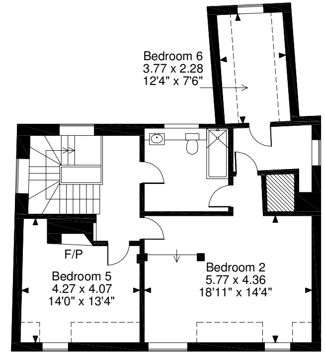
Second Floor
